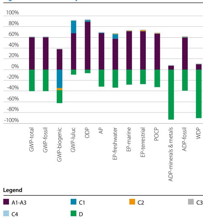
Figure 4 LCA results for Hybox® structural hollow sections
