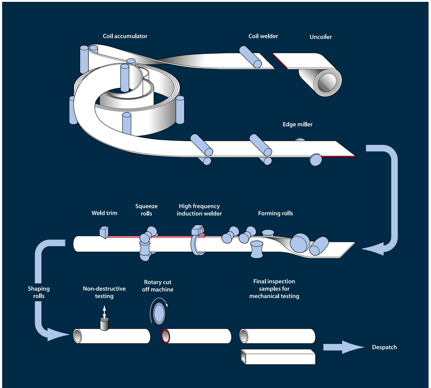
Figure 2 Process overview from hot rolled coil to cold formed structural hollow section
